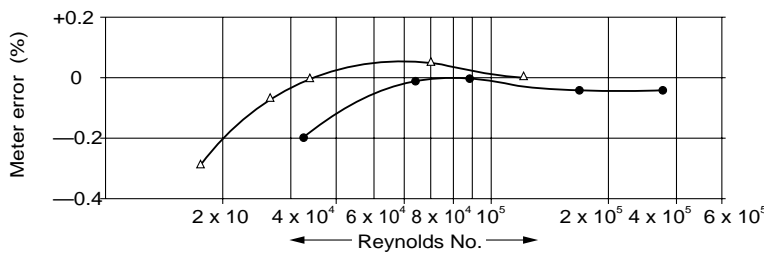
Meter Error Reynolds Numbers
