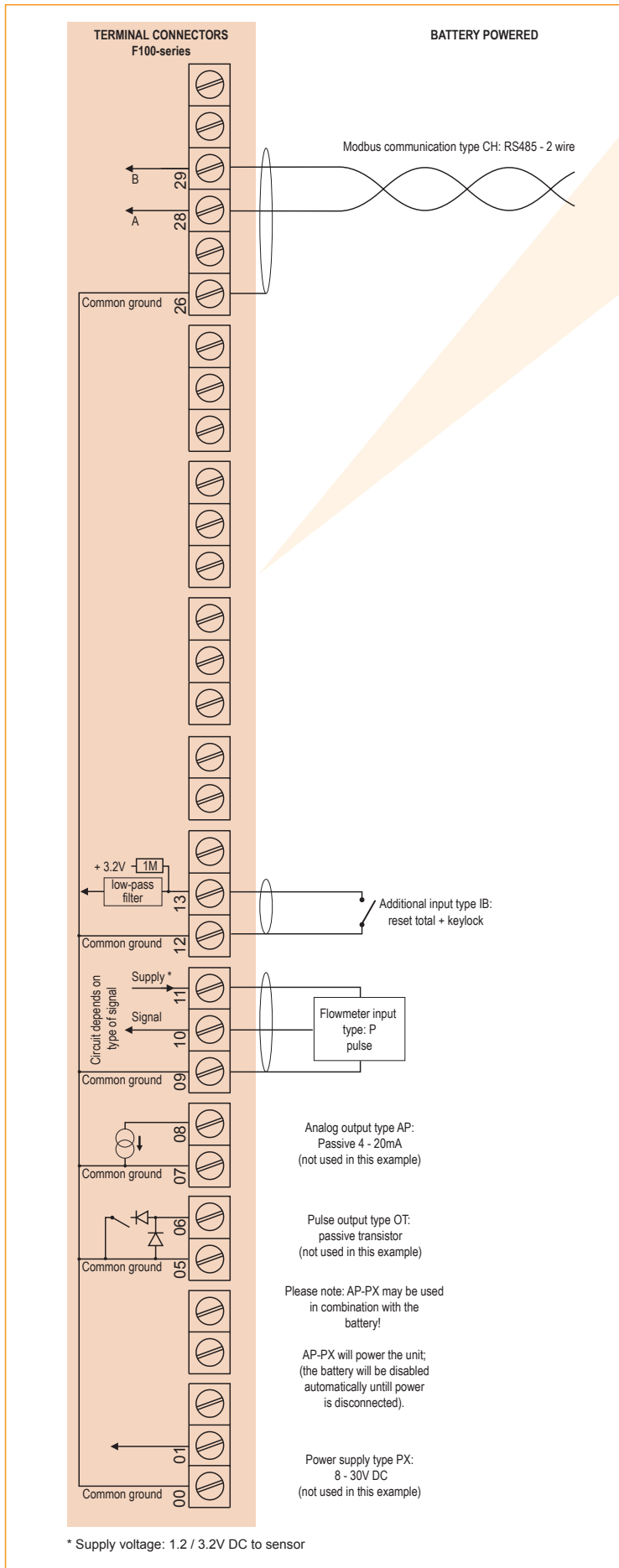
Typical wiring diagram F110-P-(AP)-CH-IB-OT-PB-(PX)
