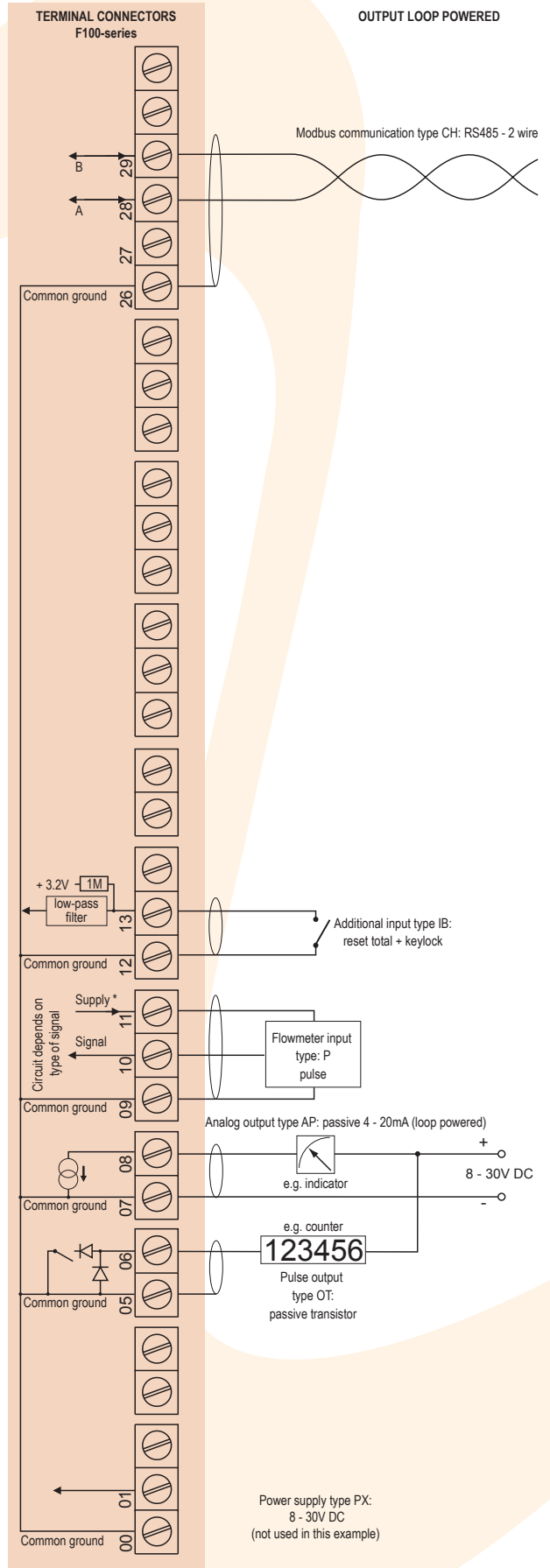
Typical wiring diagram F112-P-AP-CH-IB-OT-PX
