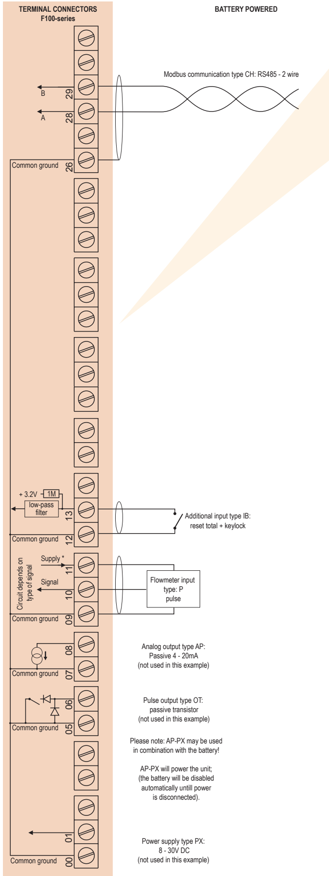
Typical wiring diagram F112-P-(AP)-CH-IB-(OT)-PB-(PX)
