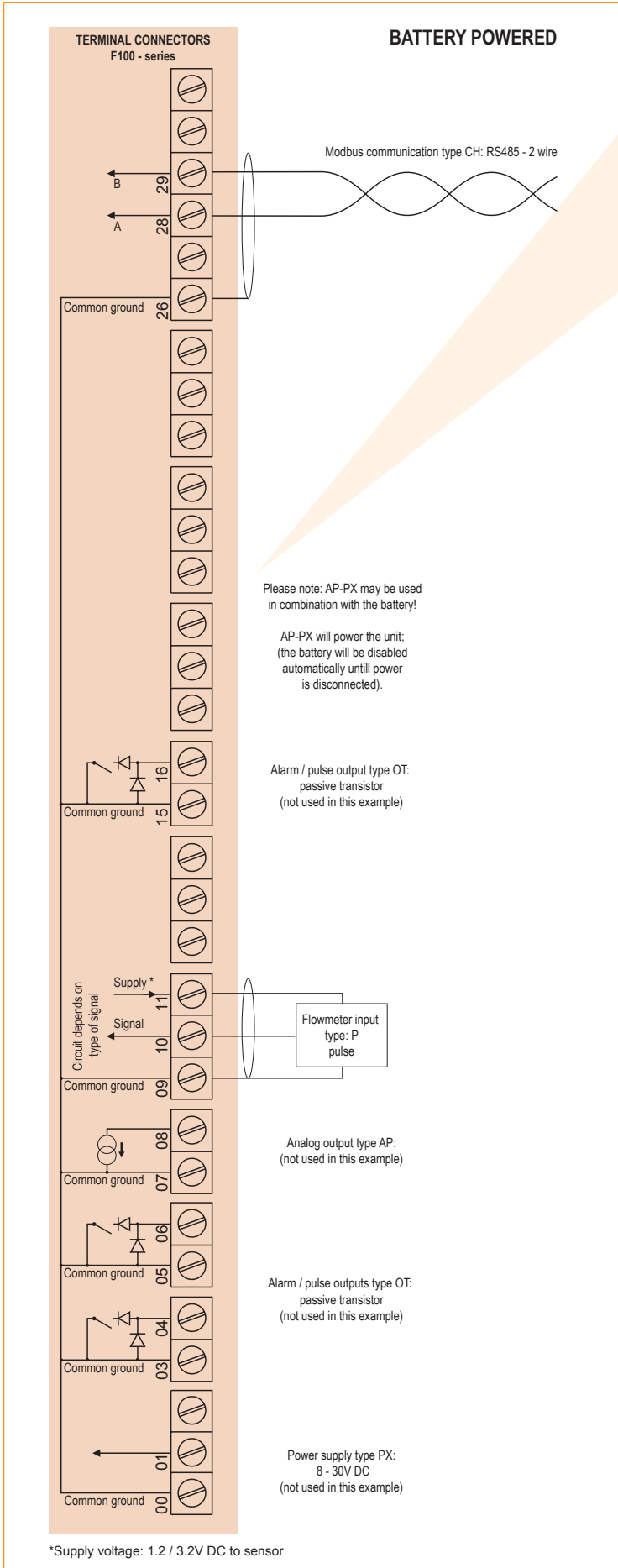
Typical wiring diagram F118-P-(AP)-CH-(OT)-PB-(PX)
