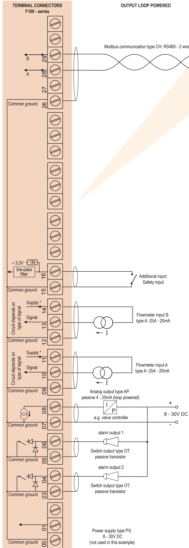
Typical wiring diagram F124-A-AP-CH-OT-(PX)
