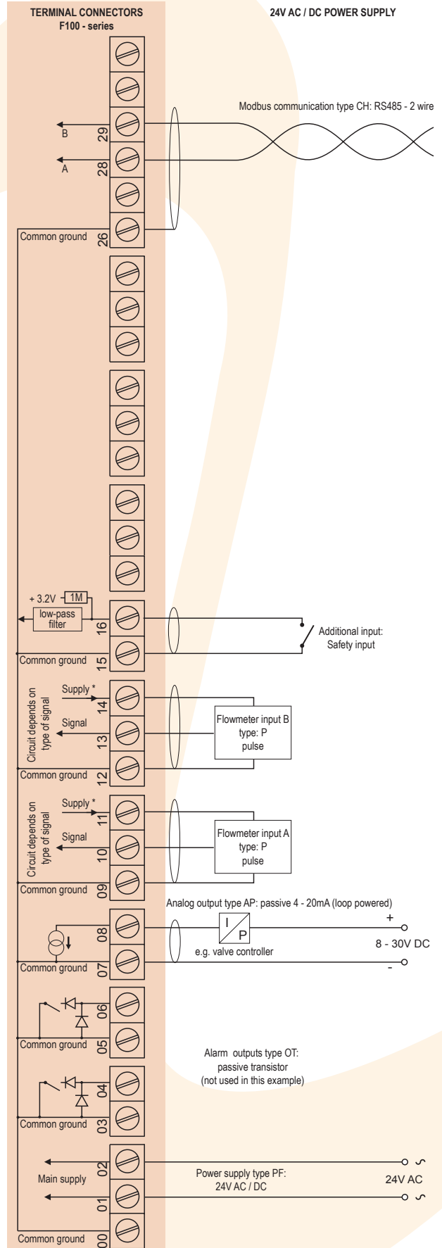
Typical wiring diagram F124-P-AP-CH-PF
