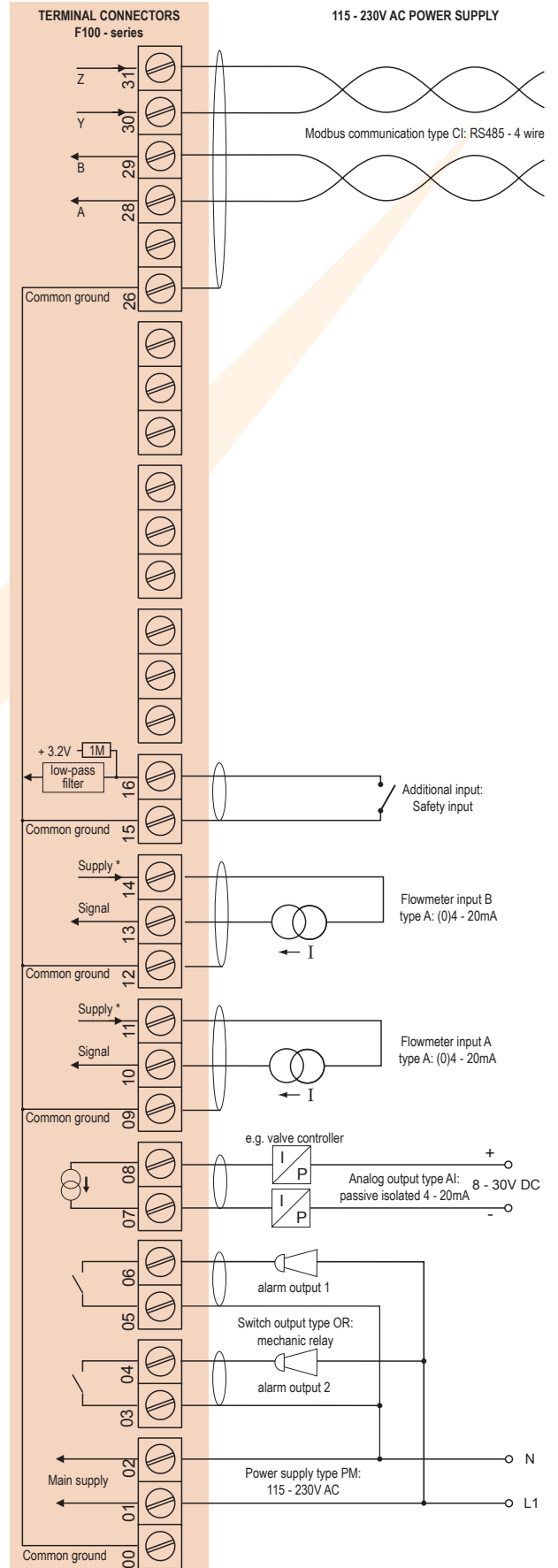
Typical wiring diagram F124-A-AI-CI-OR-PM
