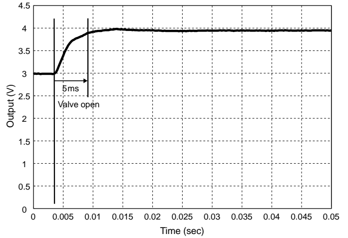
MCS100A100 output when outside valve "open" Flow rate 0 → 0.5L/min (95% response)
