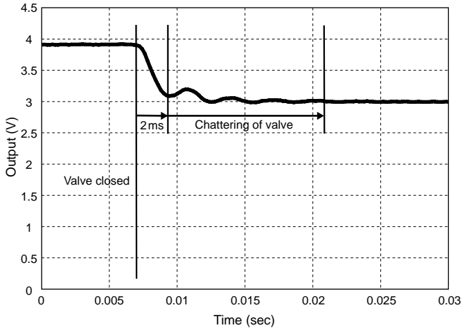
MCS100A100 output when outside valve "closed" Flow rate +0.5 → 0L/min (95% response)
