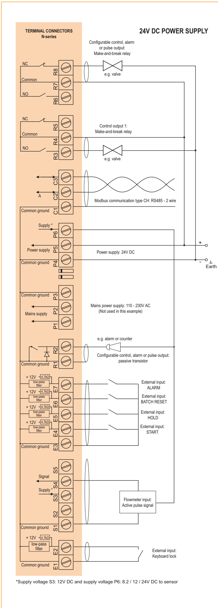
Typical wiring diagram N410-P-CH-OR-PG
